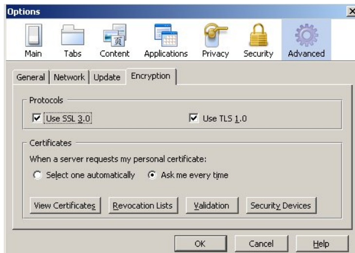
Figure 38: Firefox certificates options
