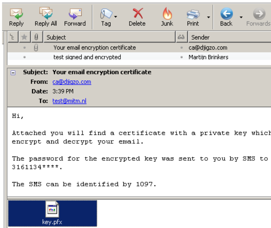
Figure 21: Thunderbird pfx attachment
